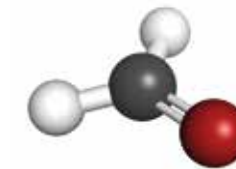
Particella Formaldeide
